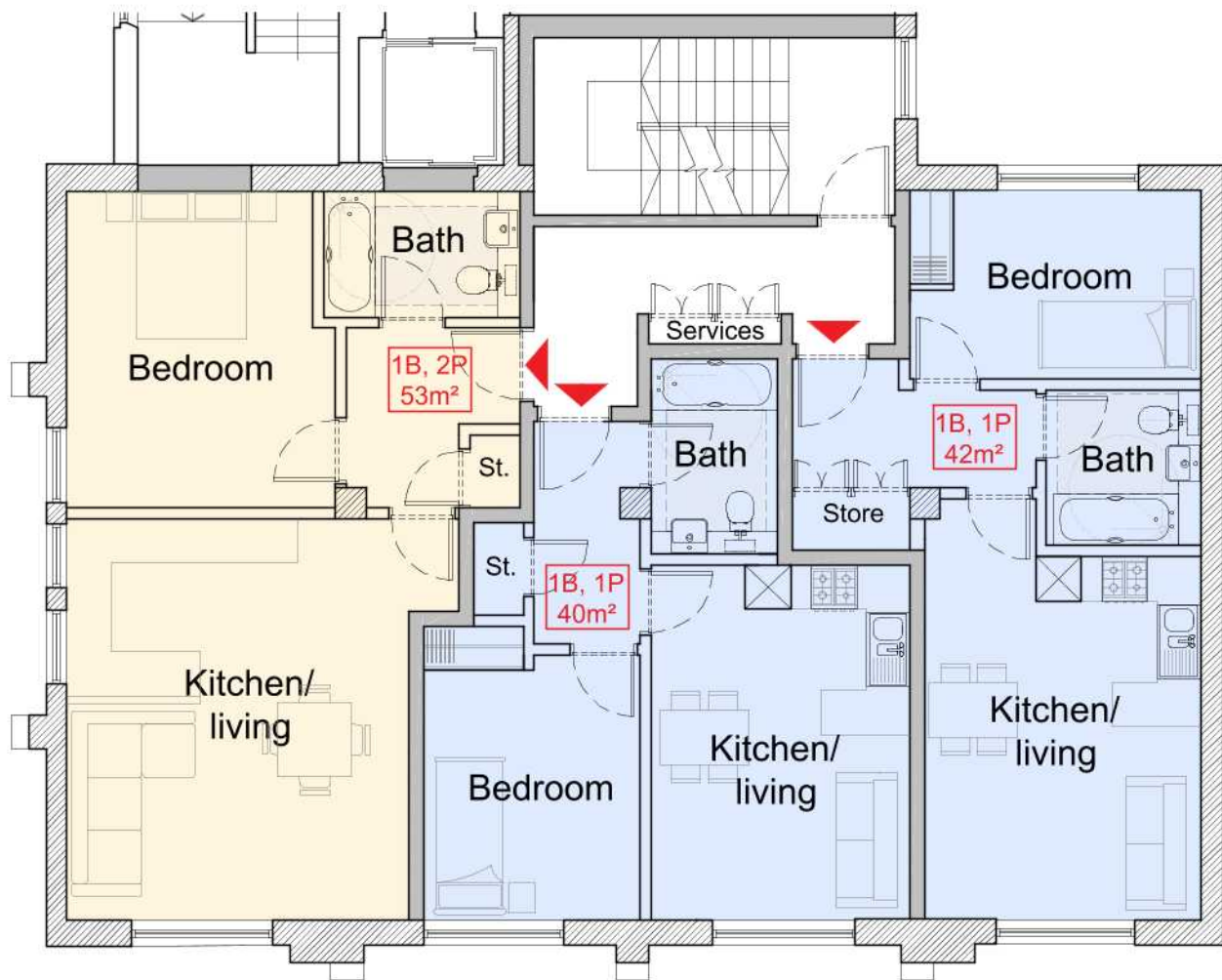
First Floor Plan 1:100
